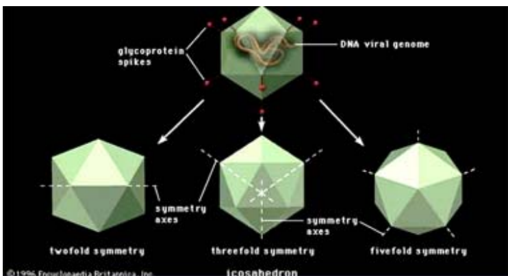
Fig.1. Example of Virion: Virus icosahedron A virus icosahedron (20-sided structure) shown in the (left) twofold, (centre) threefold, and (right) fivefold axes of symmetry. Edges of the upper and lower surfaces are drawn in solid and broken lines, respectively. Encyclopaedia Britannica
