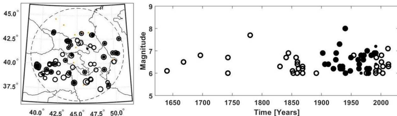
Fig. 15. Spatial and time distribution of M \geq 6 Caucasus earthquakes from 1640 to 2013 year. The location fits into a circle with a radius of 530 km. Black circles on diagrams correspond to the set of XX century 30 quakes.
