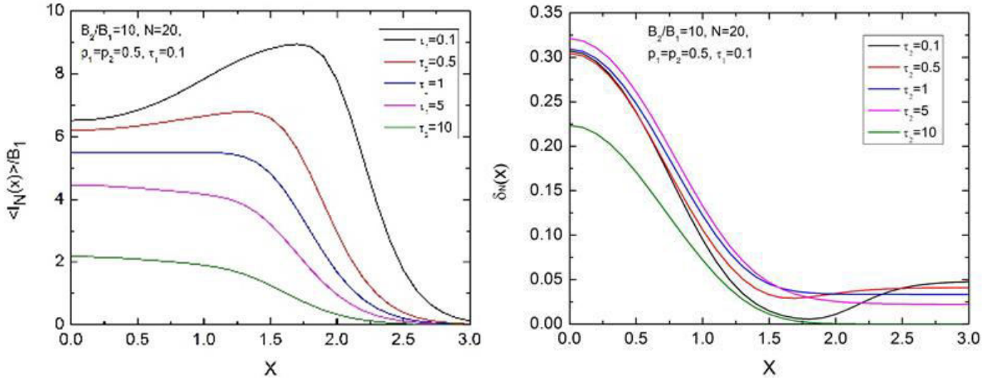
Fig.1 The statistical mean of the emitting intensities (left panel) and RelMSD (right panel) for different values of parameters. Here, a particular attention is paid to the cases of different combinations of optical thicknesses of elements.
