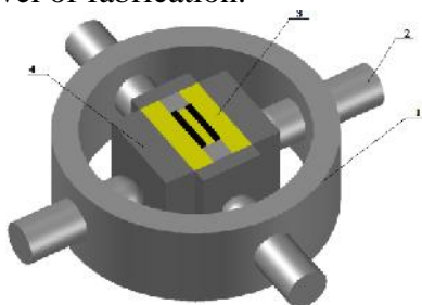
Fig. 1. The current scheme of hot pressing 1-supporting ring; 2- screws; 3- graphite mould; 4- Thermal and electrical insulators.
