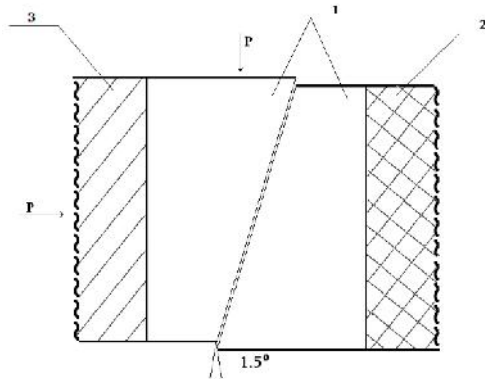
Fig. 2. Pair of conjugated cones 1-pair of cones; 2- supporting rings wall; 3- wall of mould
