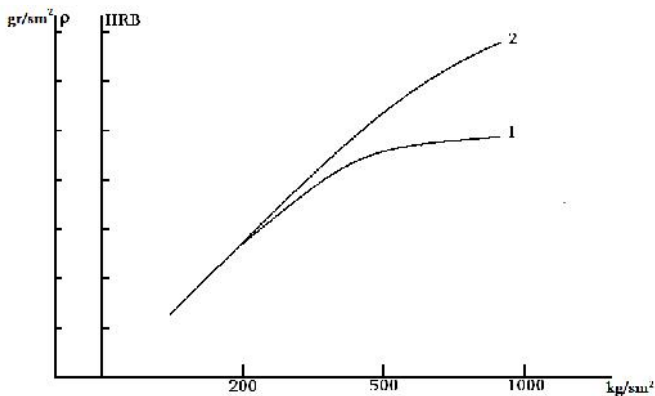
Fig. 3. Dependents of samples physical-mechanical properties on the sintering process pressure. 1-By the the current scheme (fig. 1); 2-By the developed and suggested scheme (fig. 2)
