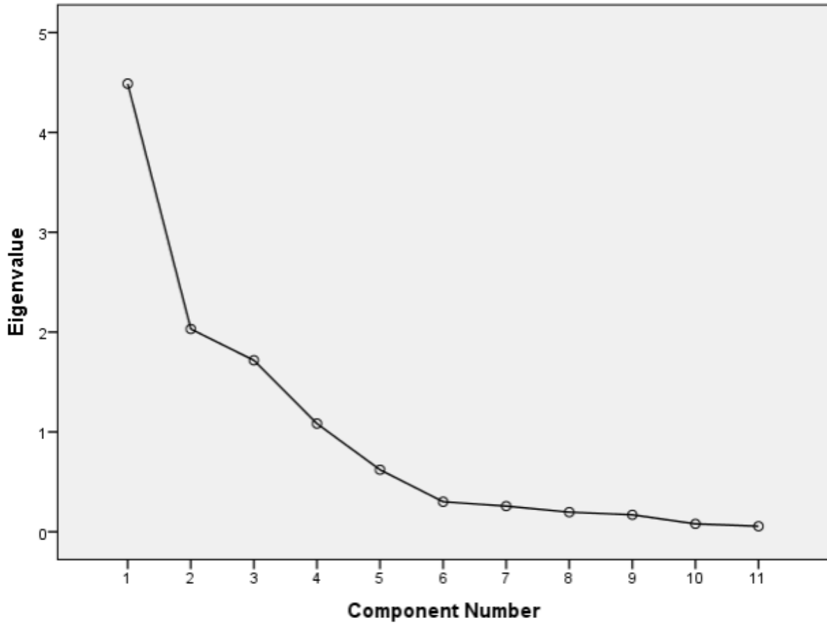
Scree Plot
