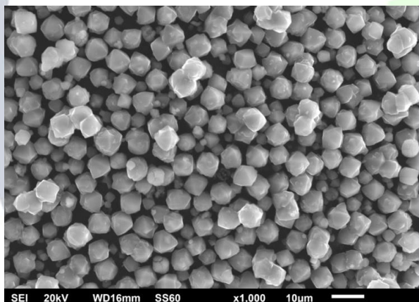
Figure 2. NaA microcrystals
