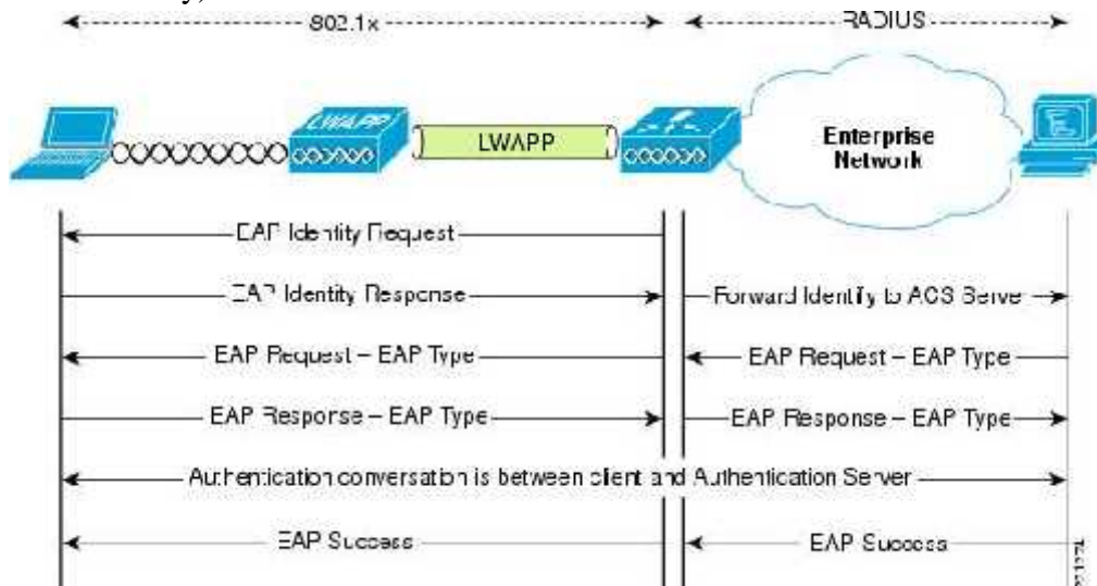
Figure 2: EAP authentication mechanism
